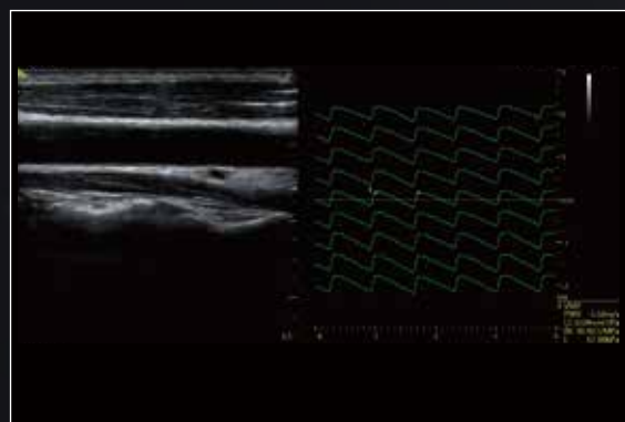
Carotid PWV
